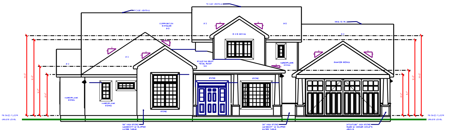
FRONT ELEVATION SCALE: 1/4" = 1'-0"
